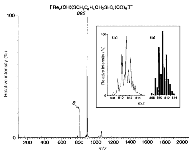
Fig. 3 Negative ion ES spectrum (cone voltage 5 V) of [Re 2 (μ-OH) 3 –(CO) 6 ] − 1 and benzene-1,4-dimethanethiol, HSCH 2 C 6 H 4 CH 2 SH, after 1 week reaction in MeCN. The inset shows a comparison of (a) experimental and (b) calculated isotope distribution patterns for the aggregate dianion 8 at m/z 811.
